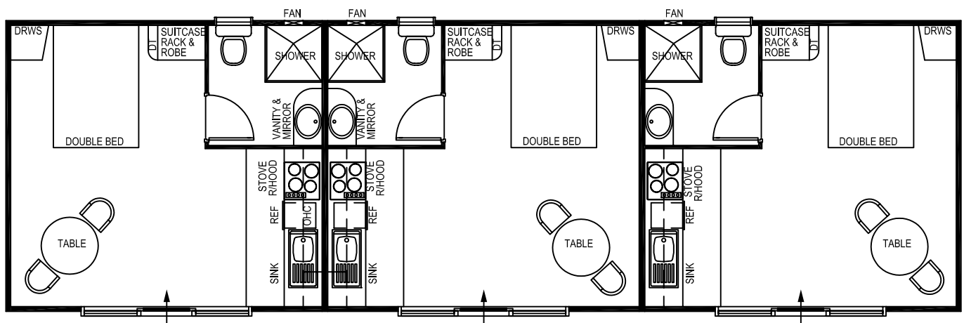
TUDOR 3 15.10x4.60 (50' x 15')
